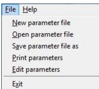
Figure 22: File Menu
