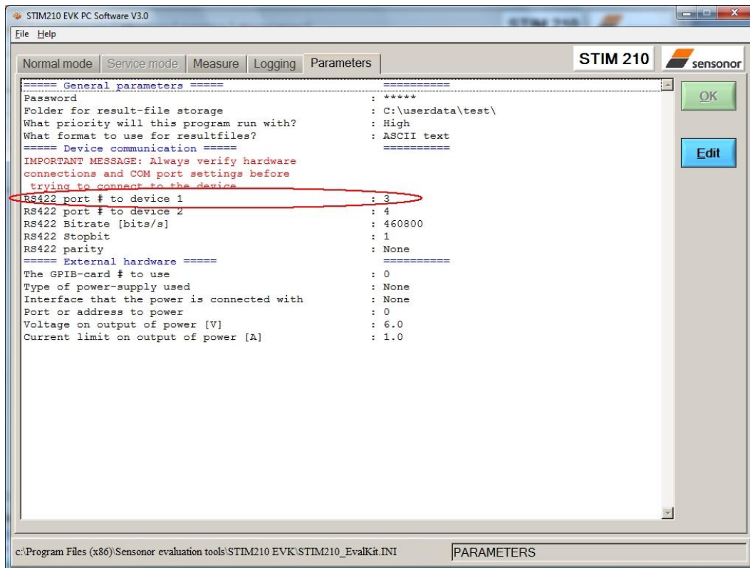
Figure 15: Editing the INI-file in order to verify the correct COM port settings
