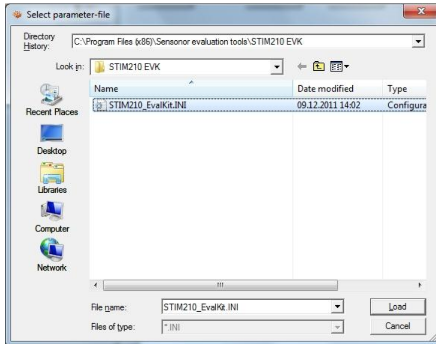
Figure 13: INI-file selection
