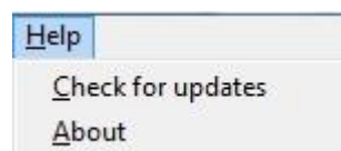
Figure 23: Help menu
