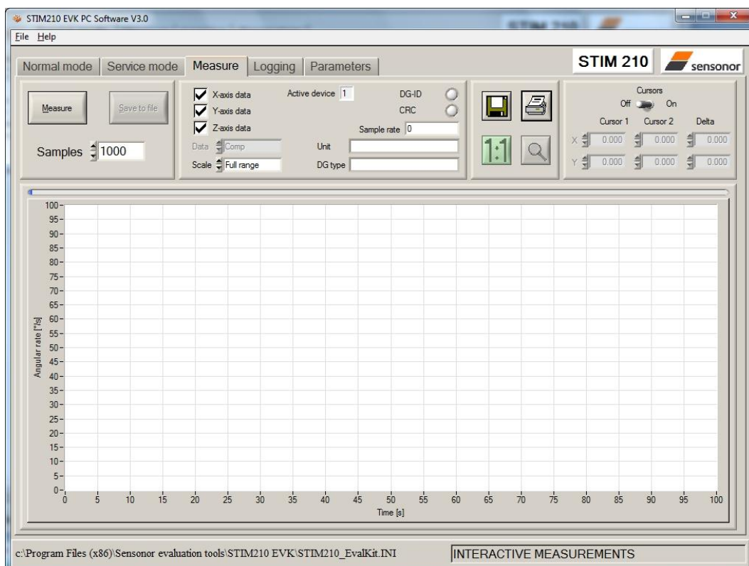
Figure 20: Measure panel
